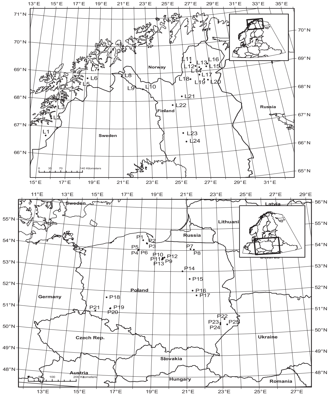
Fig. 1. Location of the studied sampling sites in Lapland and Poland.
